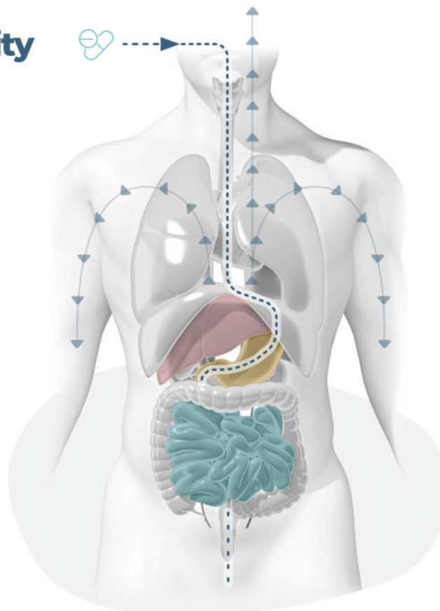
Figure 1 – Human oral bioavailability. Orally administered drugs are first solubilised by the stomach, then absorbed via the gut to be metabolised by the liver. Metabolites are then distributed through the body via transporters. Solubilised drug molecules that have not been absorbed through the gut are excreted out of the body.
