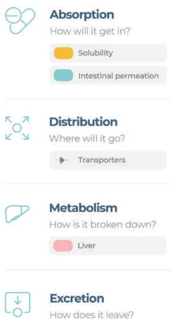
Figure 1 – Human oral bioavailability. Orally administered drugs are first solubilised by the stomach, then absorbed via the gut to be metabolised by the liver. Metabolites are then distributed through the body via transporters. Solubilised drug molecules that have not been absorbed through the gut are excreted out of the body.
