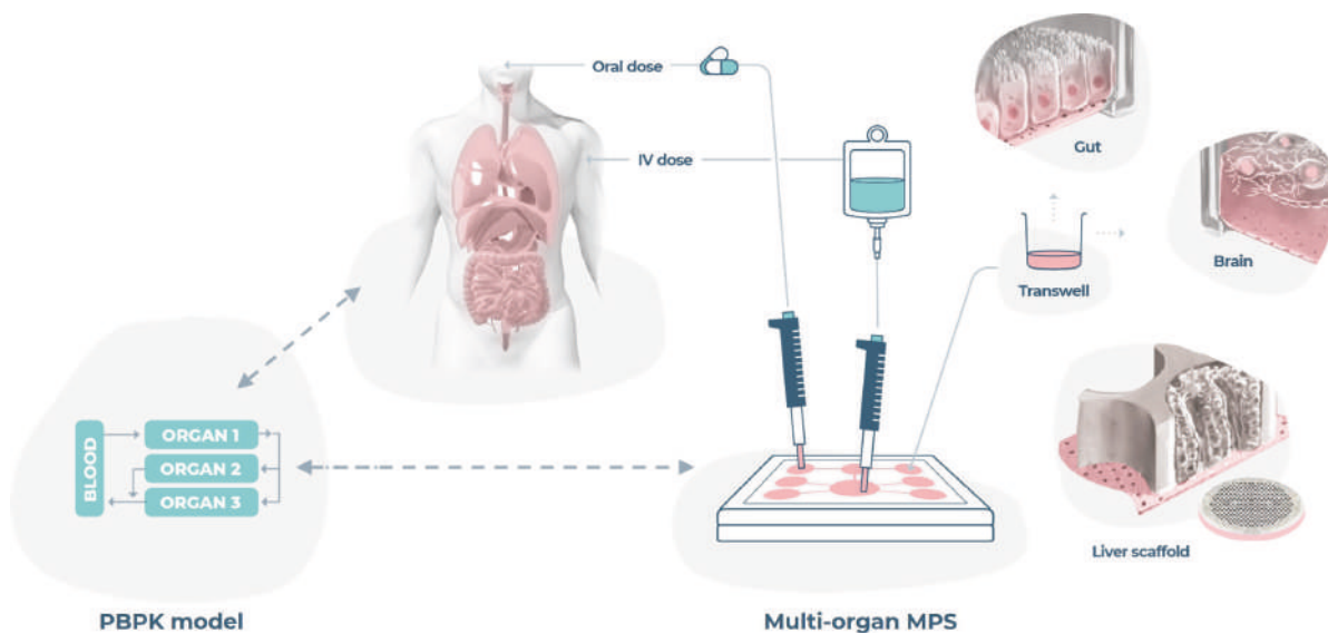
Figure 2 – Combining PBPK modelling and Organ-on-a-chip for human-relevant bioavailability
